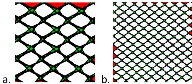
Fig. 6. Automatic and manual pores selection according to the minimum Feret diameter criteria in (a) the 10 mm x 10 mm and (b) the 24 mm x 24 mm crop sizes. The green areas indicate the pores correctly eliminated with the automatic control, while the red areas indicate the edge pores wrongly eliminated with the automatic control and included by the manual control.
