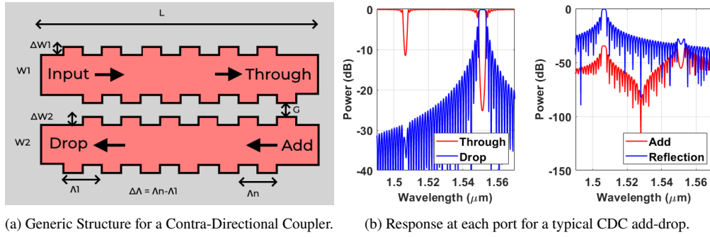
Fig. 3. Contra-DC coupler filter.
