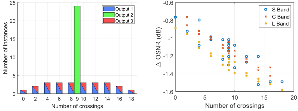
Fig. 11. Architecture penalty model, highlighting the encountered crossing distribution (a) and the calculated transmission penalty \Delta \text{OSNR} (b).
