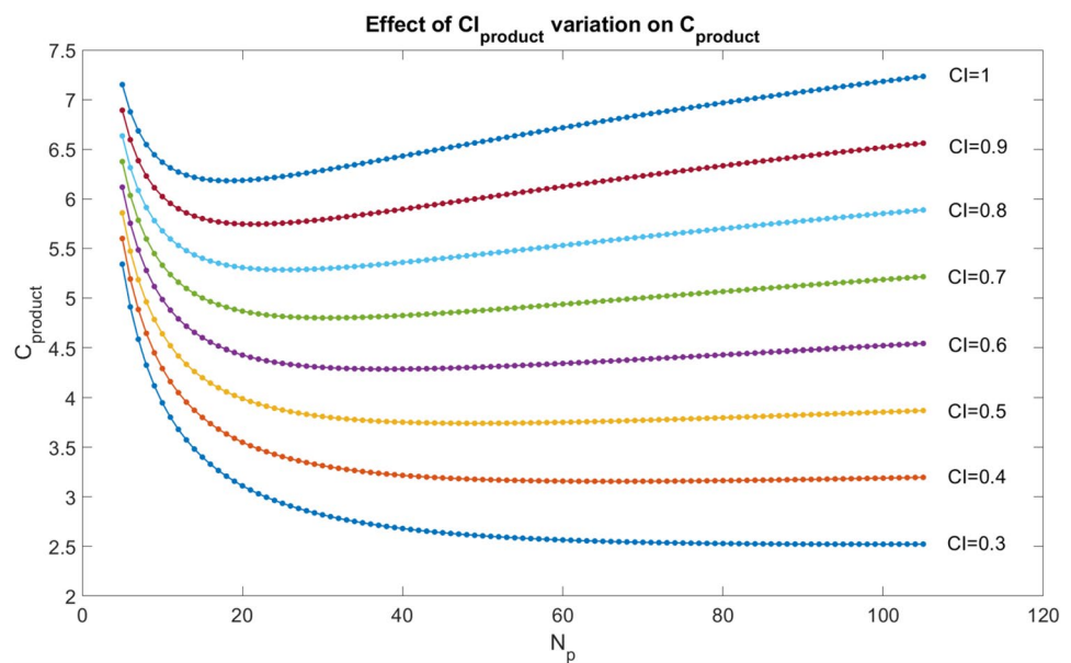
Fig. 9 Assembly complexity as function of N_p ( n_s=5 , n_p=5 , N_s=2(N_p-1) , CI_{product}=[0.3;1] )
