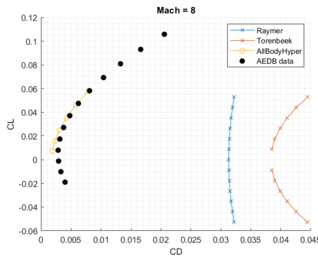
Figure 19 – C_L vs C_D curve at M = 8
