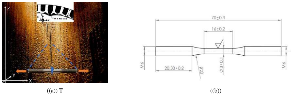
Figure 6: a) typical LRE z-axisymmetric plane fracture. 6 b) Low cycle fatigue and creep tests specimen geometry.
