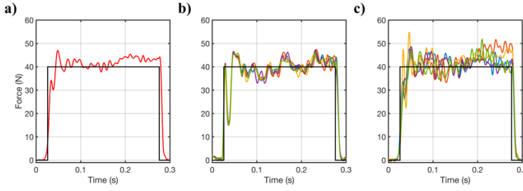
Figure 8. HuIL force tracking averaged over 5 consecutive stimuli (a). Five stimuli registered with the optimal parameter configuration in HIL (b) and HuIL (c) tests. The reference force signal is black.
