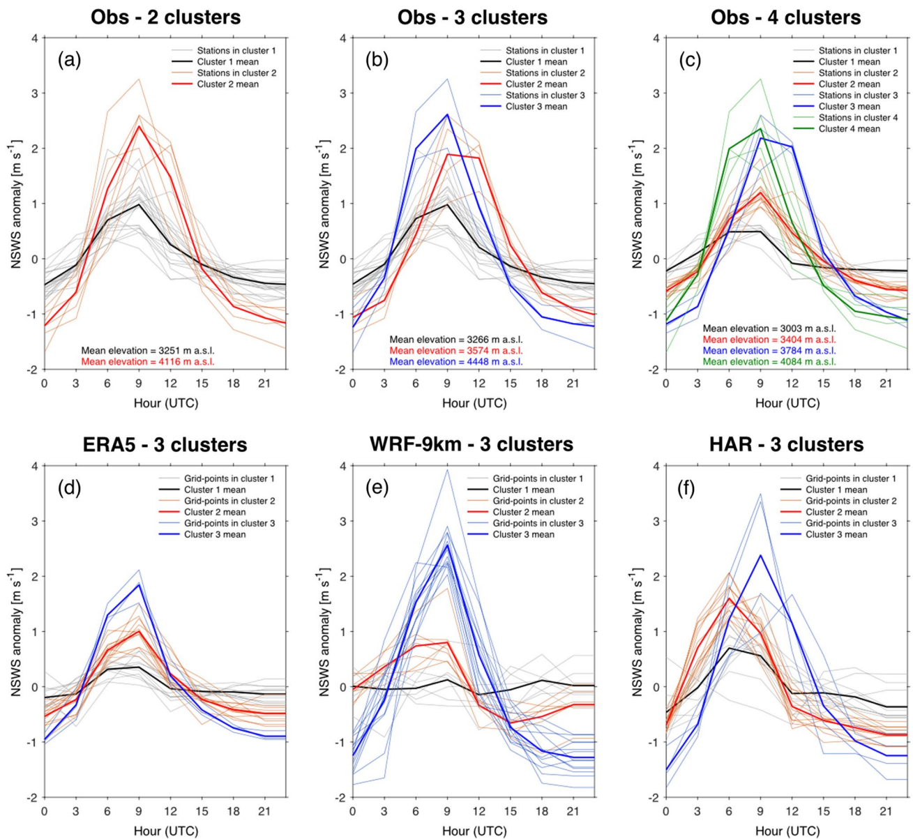
Fig. 15 Clustering of the mean 3-hourly diurnal cycle of observed and simulated NSW anomalies for 2017–2018. In particular, on the top row: Clustering of the mean 3-hourly diurnal cycle of observed NSW anomalies for 2017–2018 using 2 clusters (a), 3 clusters (b), and 4 clusters (c). On the bottom row: Clustering (with 3 classes) of the 2017–2018 mean 3-hourly diurnal cycle of NSW anomalies
