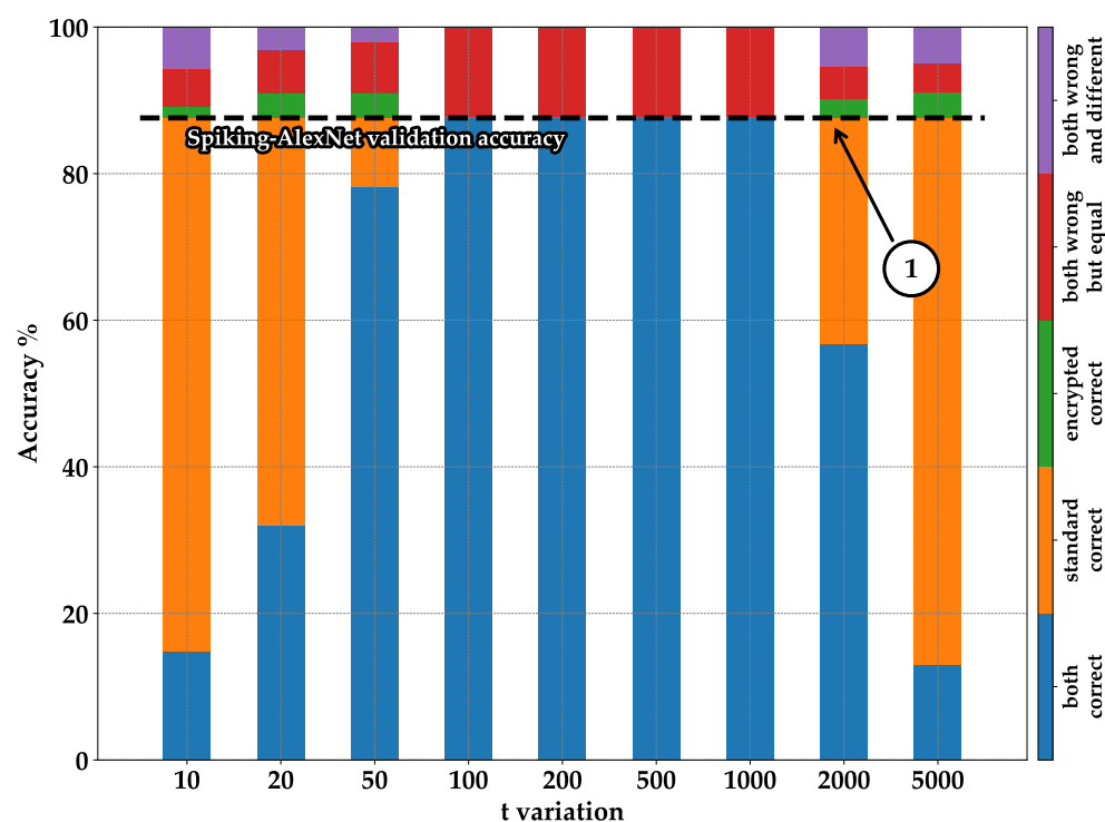
Figure 11. FashionMNIST accuracy on Spiking-AlexNet for t variation.
