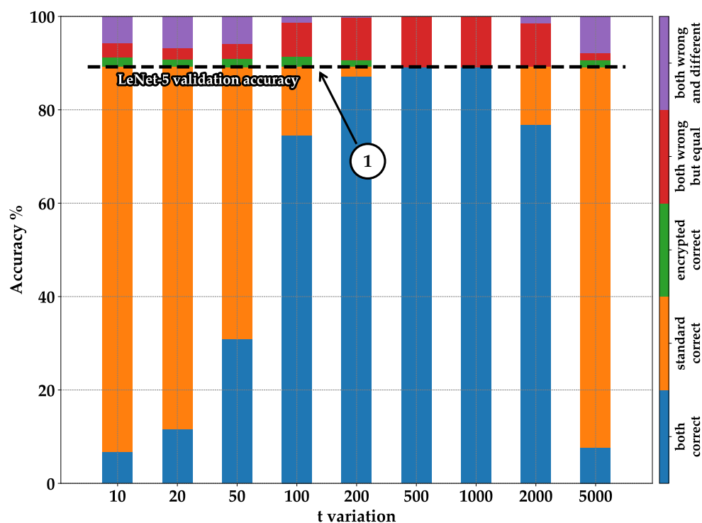
Figure 8. FashionMNIST accuracy on LeNet-5 for t variation.
