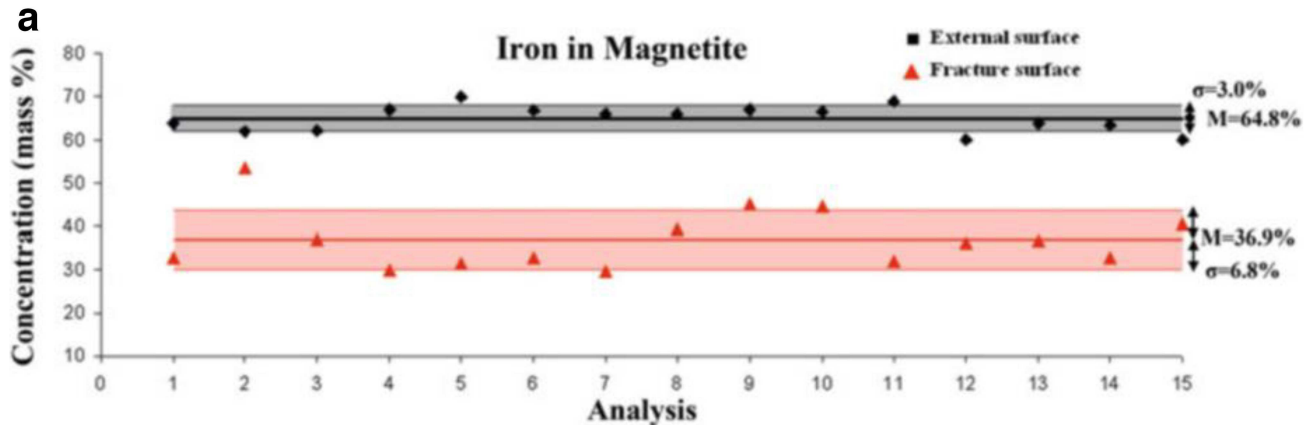
Figure 4a. Iron chemical element concentration, with mass percentages for both external and fracture surface. Fe decreased by about 27.9% in Magnetite after the brittle fracture of the specimen. The Fe concentration on the external surface was about 64.8% and the concentration on the fracture surface, after the test, was 36.9%.
