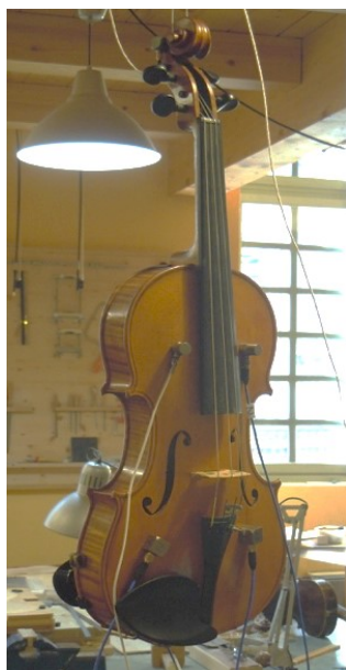
Figure 1. Set-up for the Modal Experimental Analysis.
