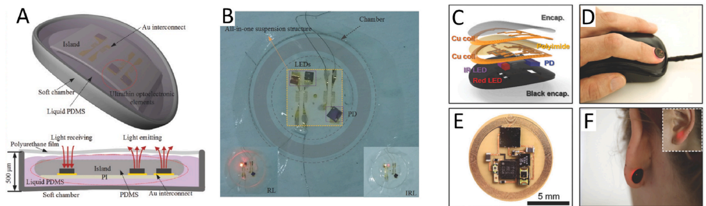
Fig. 3. A-B) Flexible photonic device for pulse oximetry developed by Li et al. Reprinted (adapted) with permission from Ref. [9]. Copyright 2023 John Wiley and Sons. C-F) Figure from Kim et al. paper. Reprinted (adapted) with permission from Ref. [10]. Copyright 2023 John Wiley and Sons. C) Scheme of the flexible photonic device for pulse oximetry developed in the work. D) Example of the device applied on the nail. E) Dimension of the device realized. F) Example of the device applied at the earlobe.
