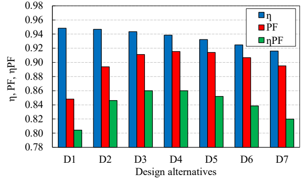
Fig. 6. The electromagnetic efficiency \eta , the power factor PF and their product \eta PF. Computations based on time-stepping FEA.
