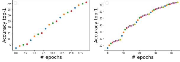
Figure 10: Evolution of classification accuracy during training with different values of N . We can see that in the first epochs of training, the accuracy on the train set presents waves with period length of size |G| . Each color represents a different classifier being trained at the given epoch for a total of |G| colors.
