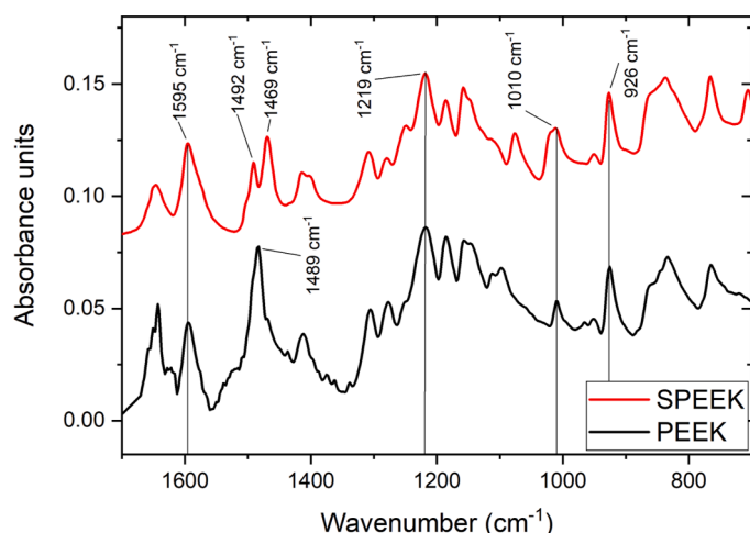
Fig. 3. ATR-IR spectra of SPEEK.
