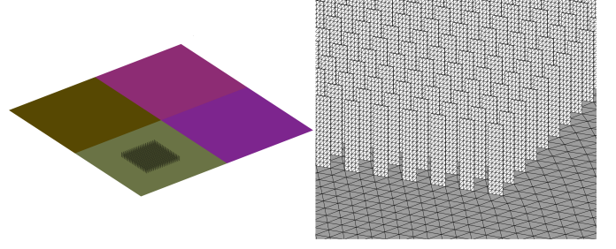
Fig. 1. Partition into subdomains and non-conformal mesh details.
