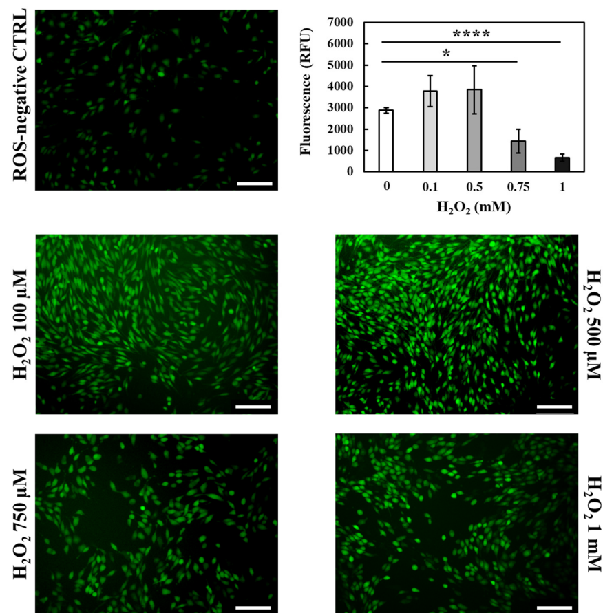
Figure 10. Qualitative and quantitative evaluation of NIH-3T3 oxidative stress induced by treating the cells with different concentrations of H_2O_2 ranging between 100 \mu M and 1 mM. Cells cultured in complete medium without the addition of H_2O_2 were used as ROS-negative control. Scale bar: 75 \mu m . Legend: **** = p < 0.0001 , * = 0.01 < p < 0.05 .
