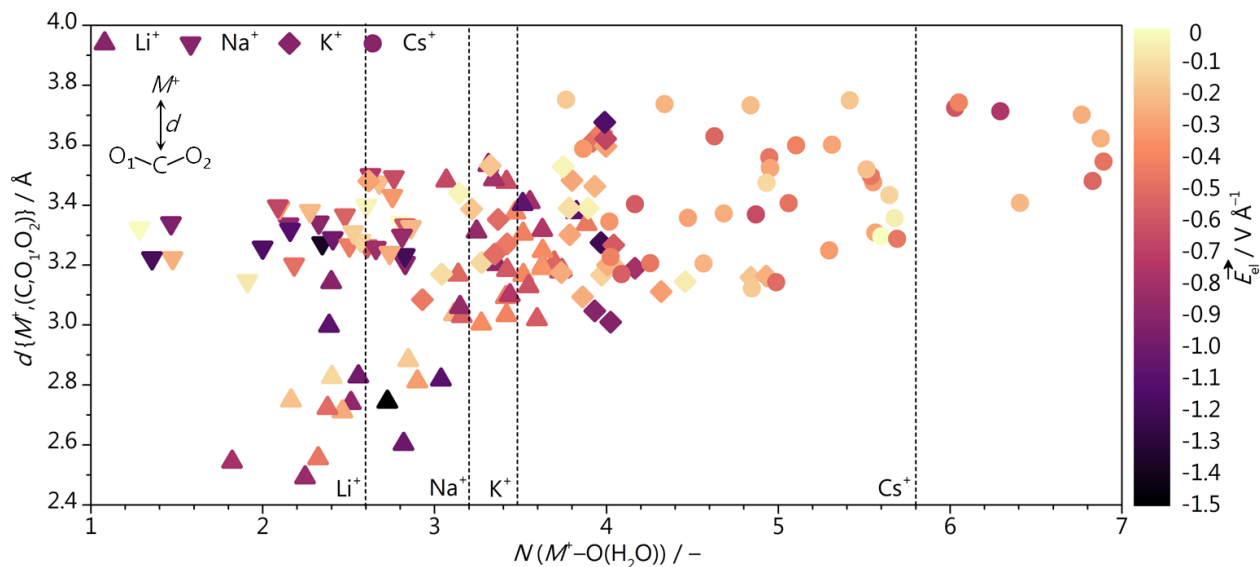
Supplementary Figure 11. Cation-induced electric field as a function of the cation-water coordination number, N(M^+ - O(H_2O)) , (horizontal axis) and the average between cation-(C, O 1 , O 2 ) distances (vertical axis) for different AIMD configurations. ▲, ▼, ◆, and ● represent Li + , Na + , K + , and Cs + respectively. Dashed lines represent average cation-water coordination numbers and are taken from Supplementary Table 2.
