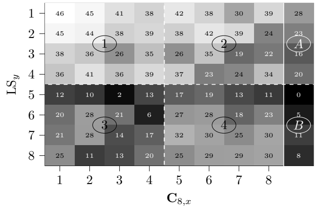
Fig. 2. Interference profile between the received code words \mathbf{C}_{8,x} for n_s = 8 and \alpha = 0.5 and the receive filters \mathbf{LS}_y . Logarithmic, values in dB. The x-axis corresponds to the indices for the received user code words, the y-axis displays the indices for the different receive filters.
