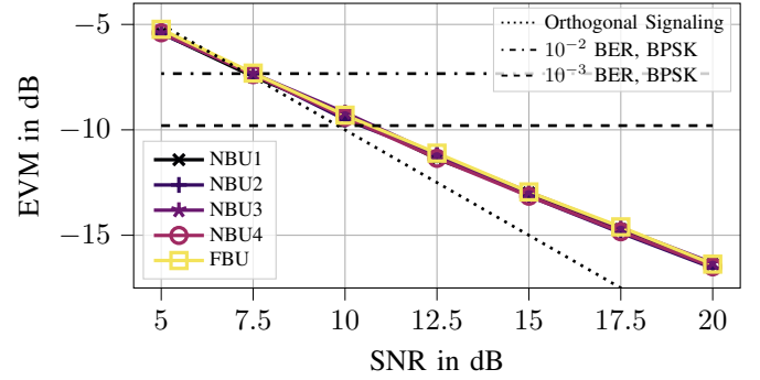
Fig. 6. EVM over SNR after Power Allocation for n_s = 8 and \alpha = 0.5 .
