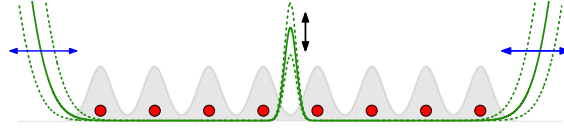
Figure 3. Pictorial representation of the parametric excitation procedure to impart energy to the TG gas, with the purpose of measuring the specific heat. The height of the barrier or the length of the guides can be modulated by changing the phase pattern on the SLM. Alternatively, the intensity of the entire pattern can be varied with an acousto-optic modulator.
