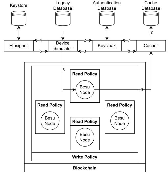
Fig. 2. Simplified architecture.
