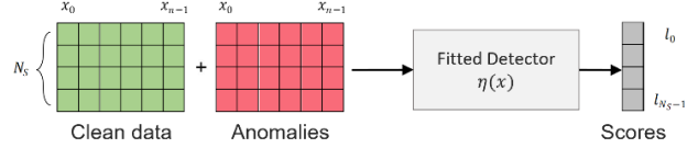
Figure 4. Inference stage
