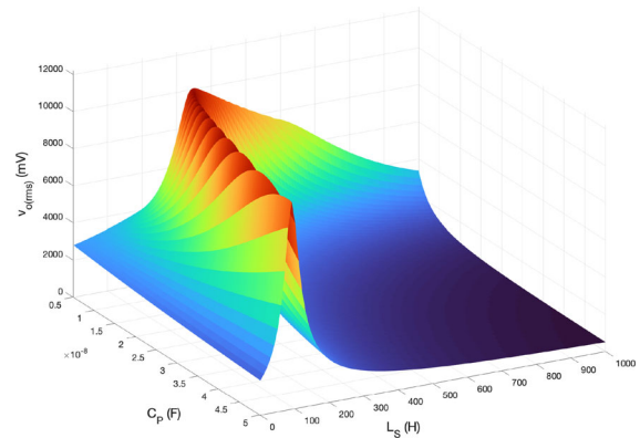
Fig. 4 Root mean square value of the output voltage v_{o(rms)} = \sqrt{E[v_0^2(t)]} vs. parameters of the matching network L_S and C_P
