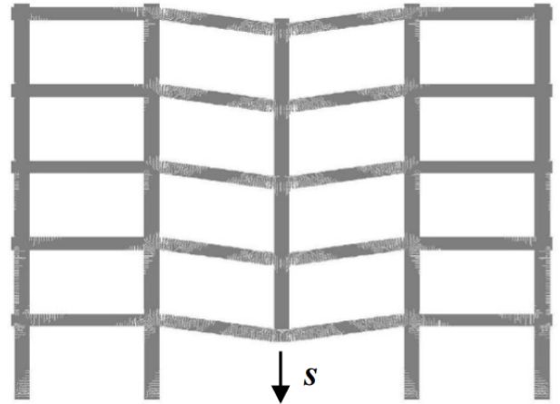
Figure 4: Scheme of the first set of non-linear static analyses: pushdown analysis.
