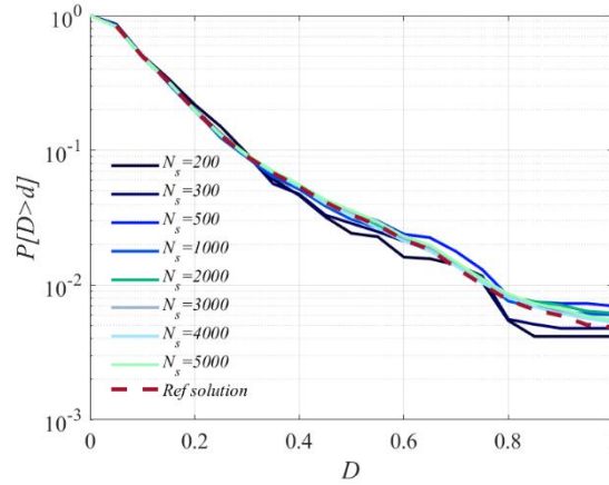
Fig. 15 Influence of number of sequences N_s on the estimate of the damage exceedance probability evaluated with the MM ( N=20 )
