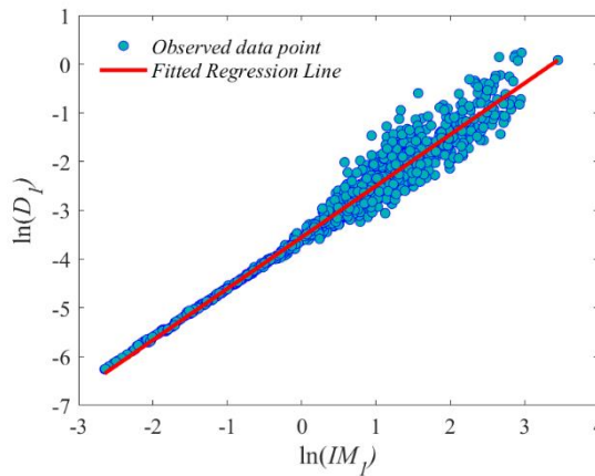
Fig. 8 Linear regression model for predicting damage after the first occurrence
