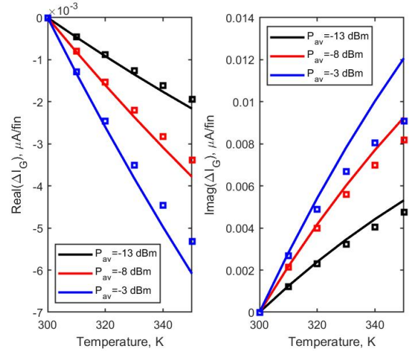
Fig. 2. Real and imaginary part of the fundamental harmonic gate current variation as a function of temperature. Lines: INC approach. Symbols: GF approach.
