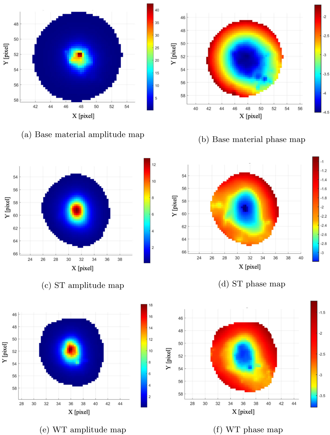
Fig. 9 Phase and amplitude maps for base material, WT and ST specimens
