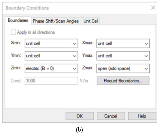
FIGURE 4. In-phase reflection characteristics simulation setup (a) geometry (b) boundary conditions.
