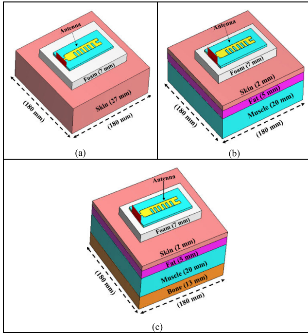
FIGURE 14. Antenna alone mounted on (a) single-layer, (b) three-layer, and (c) four-layer human body models at x = 0.05\lambda_0 .
