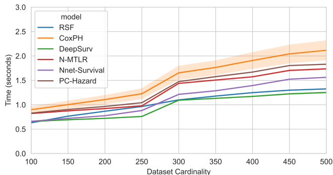
Fig. 2. Execution time for each model on several cuts of the GBSG2 dataset. For neural models, time refers to 300 epochs. Results are averaged over 100 runs.
