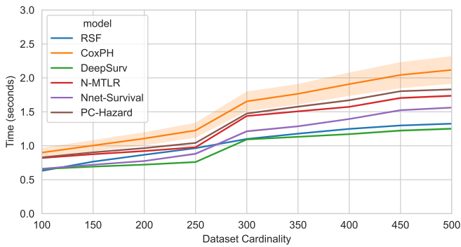
Fig. 2. Execution time for each model on several cuts of the GBSG2 dataset. For neural models, time refers to 300 epochs. Results are averaged over 100 runs.
