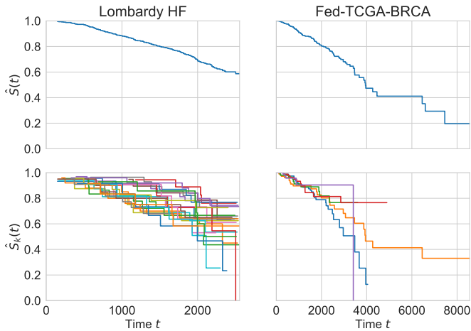
Fig. 4. Kaplan-Meier estimators \hat{S}(t) for datasets of real-world federations. The first row shows KM estimators for the entire dataset, while the second row depicts a KM curve for each client k .
