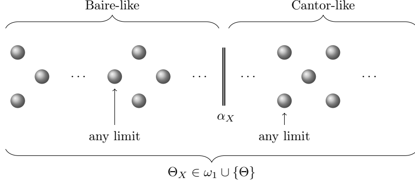
FIGURE 3. The Wadge hierarchy \mathcal{W}_X on an arbitrary zero-dimensional Polish space X when \mathcal{W}_X is isomorphic neither to \mathcal{W}_{\mathcal{N}} nor to \mathcal{W}_{\mathcal{C}} . In this case, the ordinal \alpha_X satisfies \omega < \alpha_X < \omega_1 .
