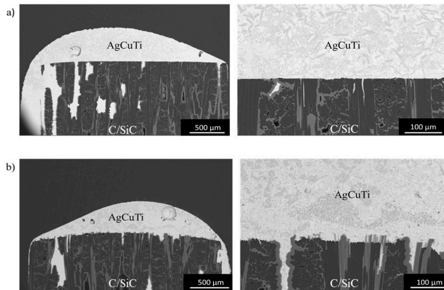
Fig. 7. Cross-sections of CB4 wetted C/SiC after wetting tests: untreated (a) and 30s APPJ treated (b) C/SiC. Micrograph was taken in BSE mode.
