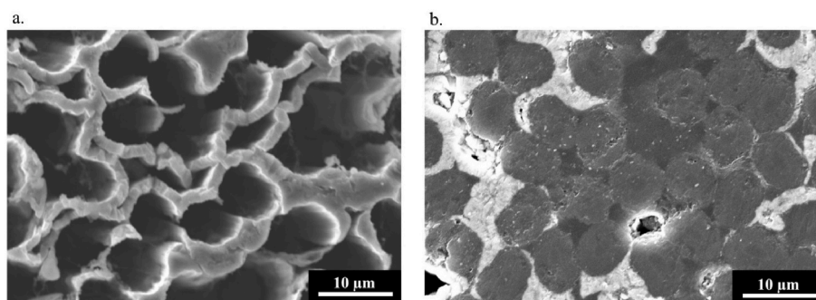
Fig. 2. 5 min APPJ-treated C/SiC: exposed surface (a) and an internal surface taken 400 \mu\text{m} below (b).
