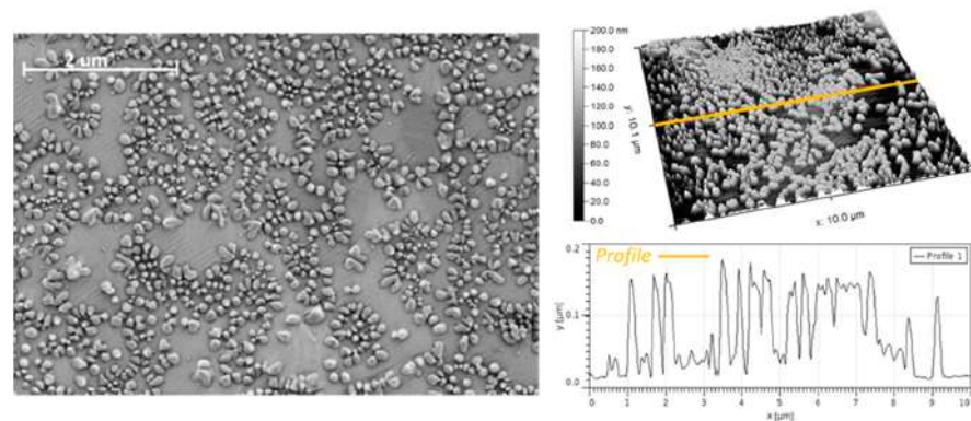
Figure 4. 43 kX FESEM image of the surface of the direct growth sample (on the (left) ); 10 \mu\text{m} \times 10 \mu\text{m} AFM height map in the centre of the sample coated with direct growth graphene (on the (right) ). The line profile shows the characteristic dimensions of the globular structure.
