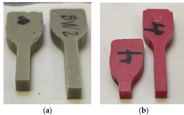
Figure 5. Adhesive dogbone failure surfaces: (a) polyurethane (ADEKIT A 236/H 6236); (b) epoxy (SIKAPOWER-1277).
