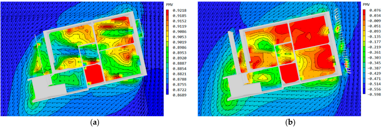
Figure 14. Phoenix 2019 software simulation results: (a) PMV (before renovation); (b) PMV (after renovation).
