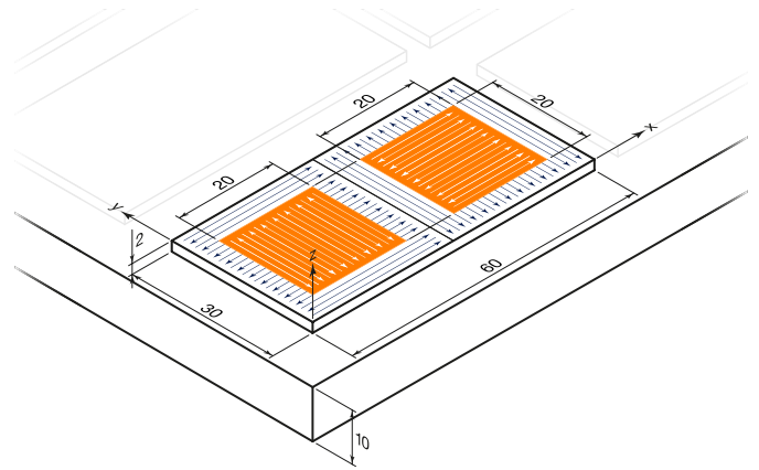
Fig. 1. Geometry and dimensions of the deposited sample, and the laser polishing area locations.
