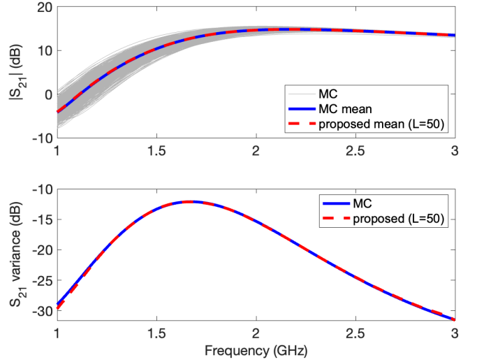
Fig. 3. S_{21} parameter of the LNA in Fig. 1. Top panel: the gray lines show the magnitude of the S_{21} computed from a 1000-sample MC simulation. The blue solid and the red dashed lines are the magnitude of the average S_{21} obtained from the MC samples and the proposed models, respectively. Bottom panel: the blue solid and the red dashed lines are the magnitude of the S_{21} variance obtained from the MC samples and the proposed models, respectively.
