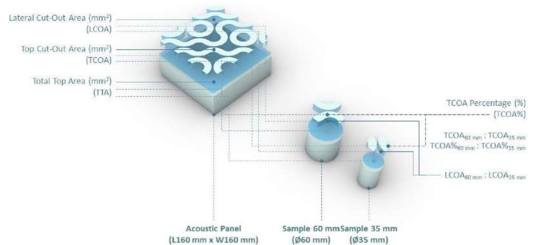
Figure 7. The TCOAs, LCOAs, and TTAs on rectangular acoustic panels, 60 mm samples, and 35 mm samples. The TCOAs 60 mm and TCOAs 35 mm evaluated as a percentage with respect to the TTA of the respective cylindrical specimens.
