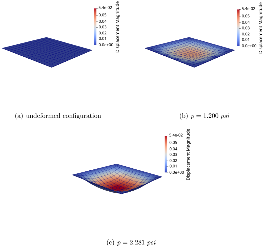
Figure 13: Undeformed and deformed states of the silicone rubber plate.
