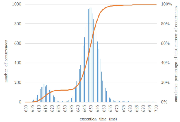
Fig. 10. Number of executions completed in a given amount of time for 8 real banknotes.
