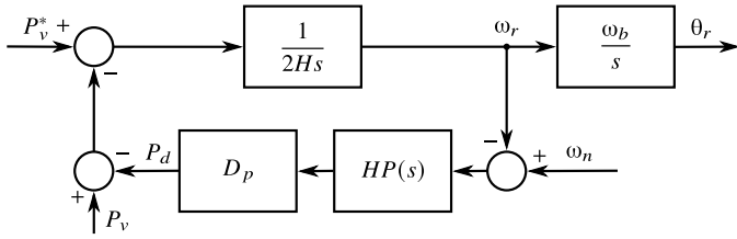
Fig. 8. Diagram of the mechanical emulation block with the High-Pass droop-based damping.
