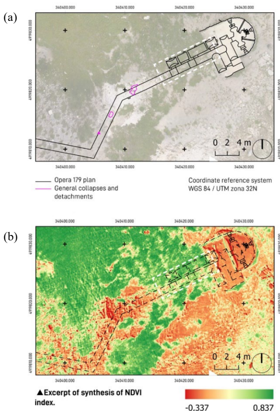
Figure 7. Comparison between visible orthophoto (a) and NDVI map (b) with the identification – in white - of corridor of opera 179.
