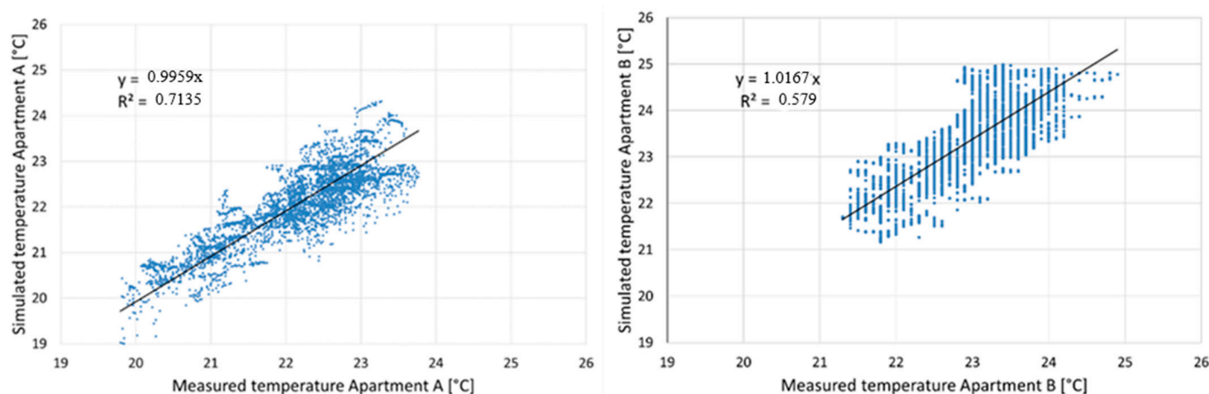
Figure 10. UniTN calibrated model—apartment A (left) and B (right): simulated vs. measured temperature; the linear interpolation (black line) and the corresponding equation are shown.
