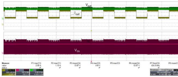
Fig. 10: Switching waveforms at dynamic load variation in steady-state operation. V_{DS}=100V/div , I_{out}=500mA/div , V_{out}=5V/div , t=160ms/div
