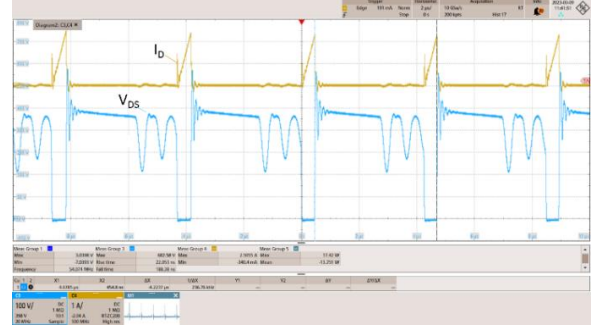
Fig. 11: GaN FET switching waveforms in steady state at V_{out}=14V , I_{out}=3A . V_{DS}=100V/div , I_D=1A/div , t=2\mu s/div
