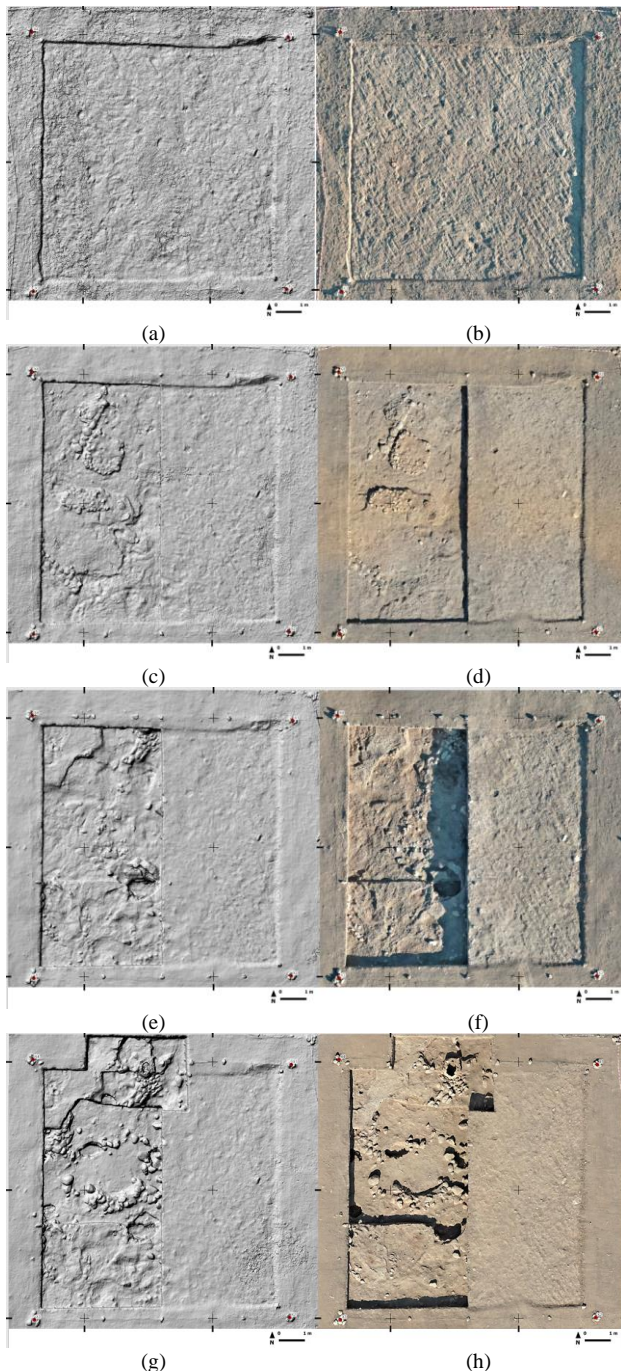
Figure 7. A sample of epochs results, DSM, left and ortho, right: (a) and (b) for 25/09; (c) and (d) for 26/09; (e) and (f) for 10/10; (g) and (h) for 16/10.
