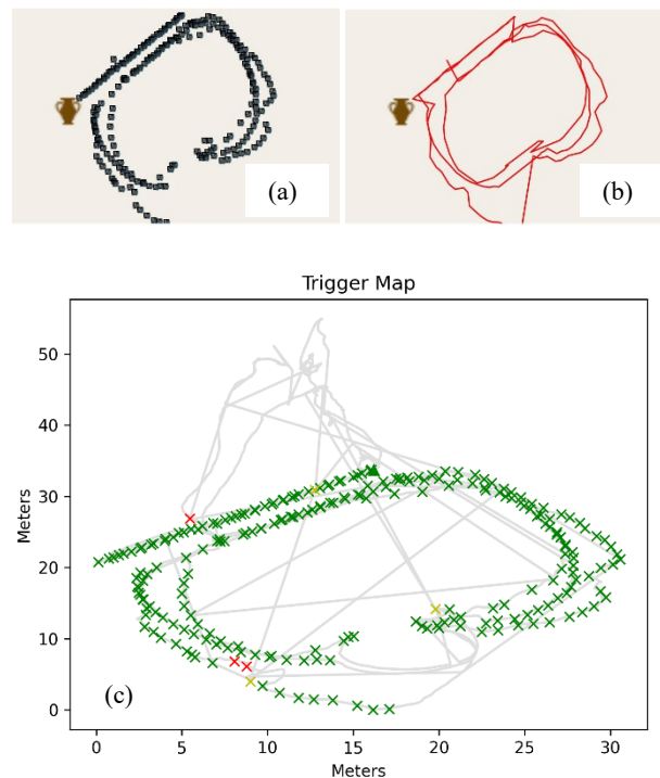
Figure 9. Postprocessing of the acquired images of the 3D ImageVector using the REDtoolbox software. Position of the geotagged images (a), IMU track (b) and trigger map (c) of the Mezzagnone test site
