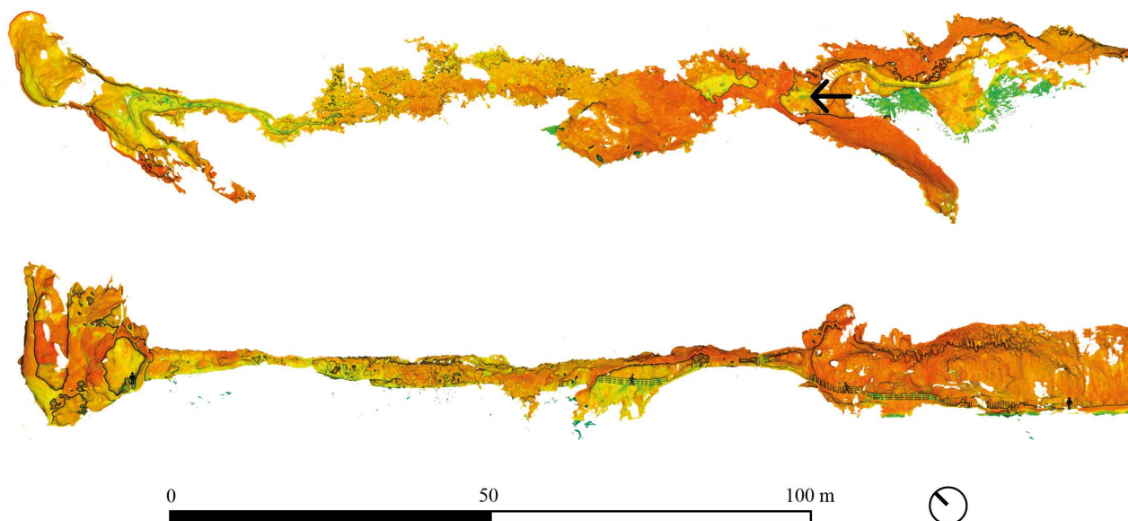
Figure 9. Plan and section of the obtained STONEX® X120 GO SLAM Laser Scanner point cloud (Dataset 1). The point cloud is displayed with the Intensity value as point colour and the black arrow states the cave entrance.
