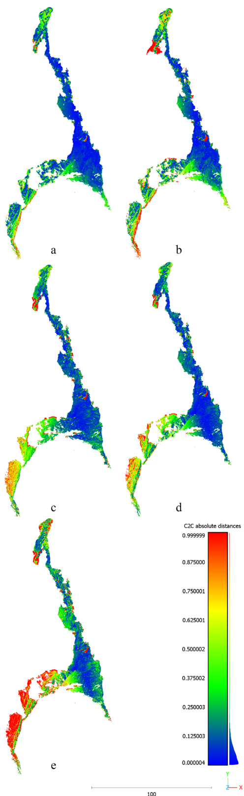
Figure 11. C2C comparison between the Dataset 1 (STONEX® X120GO SLAM Laser Scanner) and the LiDAR data (FARO Focus3D X330). The (a) image shows the evaluation of the point cloud computed with Stability value set at 1, the (e) is referred to the one processed with the Stability value set at 5.
