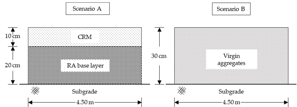
Figure 1. Cross-sections corresponding to the considered scenarios.
