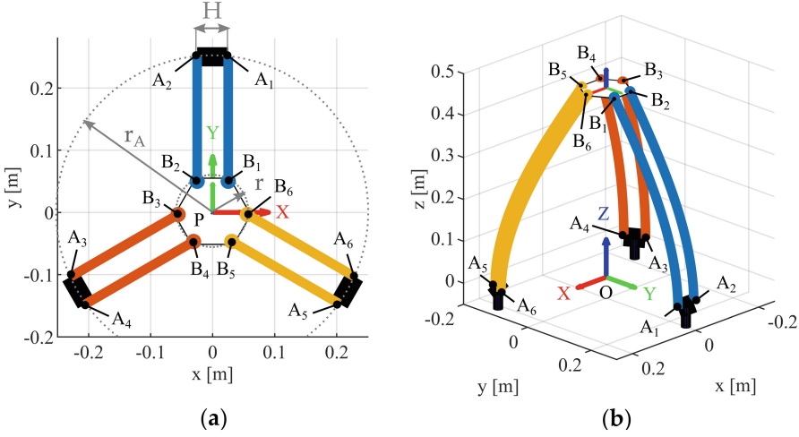
Fig. 2. Architecture 2: Flexible Tripod 3PFSS with parallel rods and fixed rod length: (a) top view and geometric parameters definition, (b) 3D representation.
