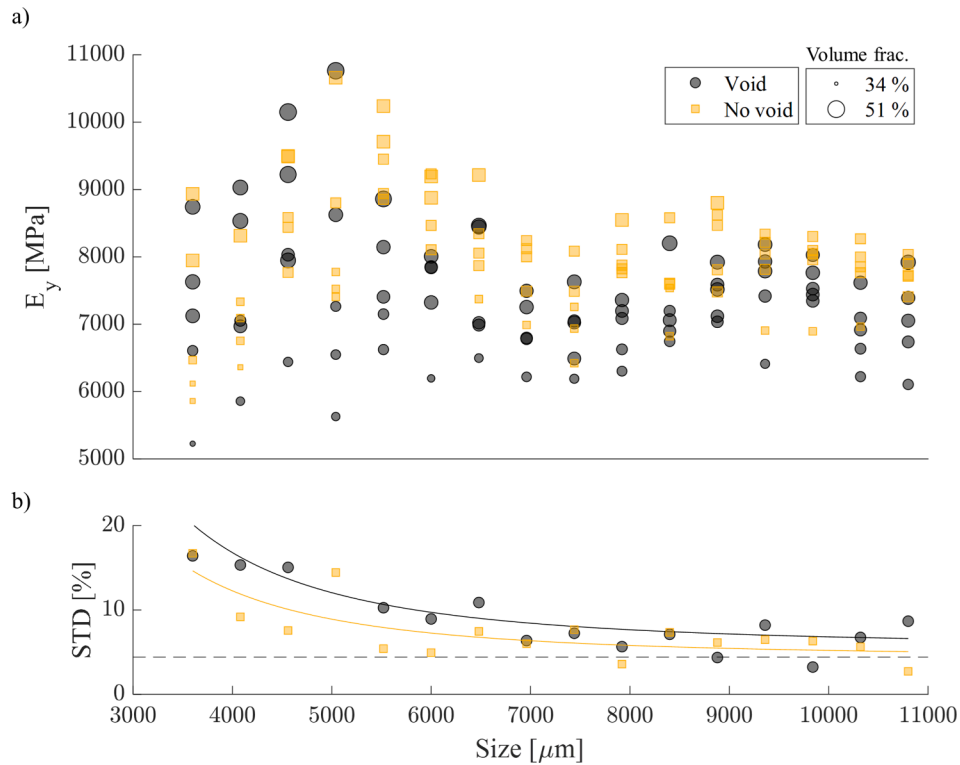
Fig. 10. On top, the homogenized modulus computed with FFT simulations of reconstructed microstructures, on the bottom, the standard deviation normalized to the mean.
