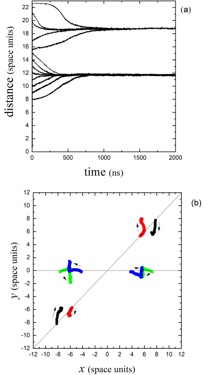
FIG. 3. Interaction of two CSs far from the locking point ( |E_{HB}|^2 = 0.75 ). (a) Time evolution of the distance of pairs of CSs with different initial distance; (b) trajectory of the CSs for initial distance equal to 21.21 (black), 15.56 (red), 15 (green), and 8 (blue). The CSs merge when the initial distance is smaller than 8 s.u.
