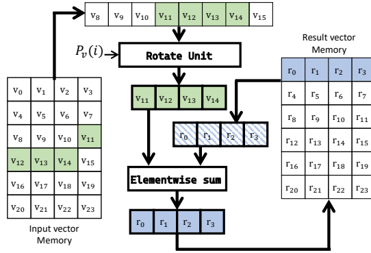
Fig. 1. VbC with n_b = 4 .
